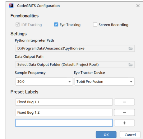
Figure 2: Configuration panel of CodeGRITS.
